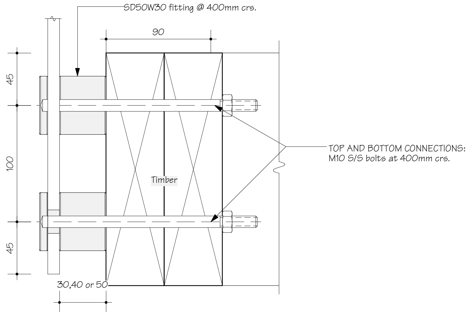
TIMBER FIXING
