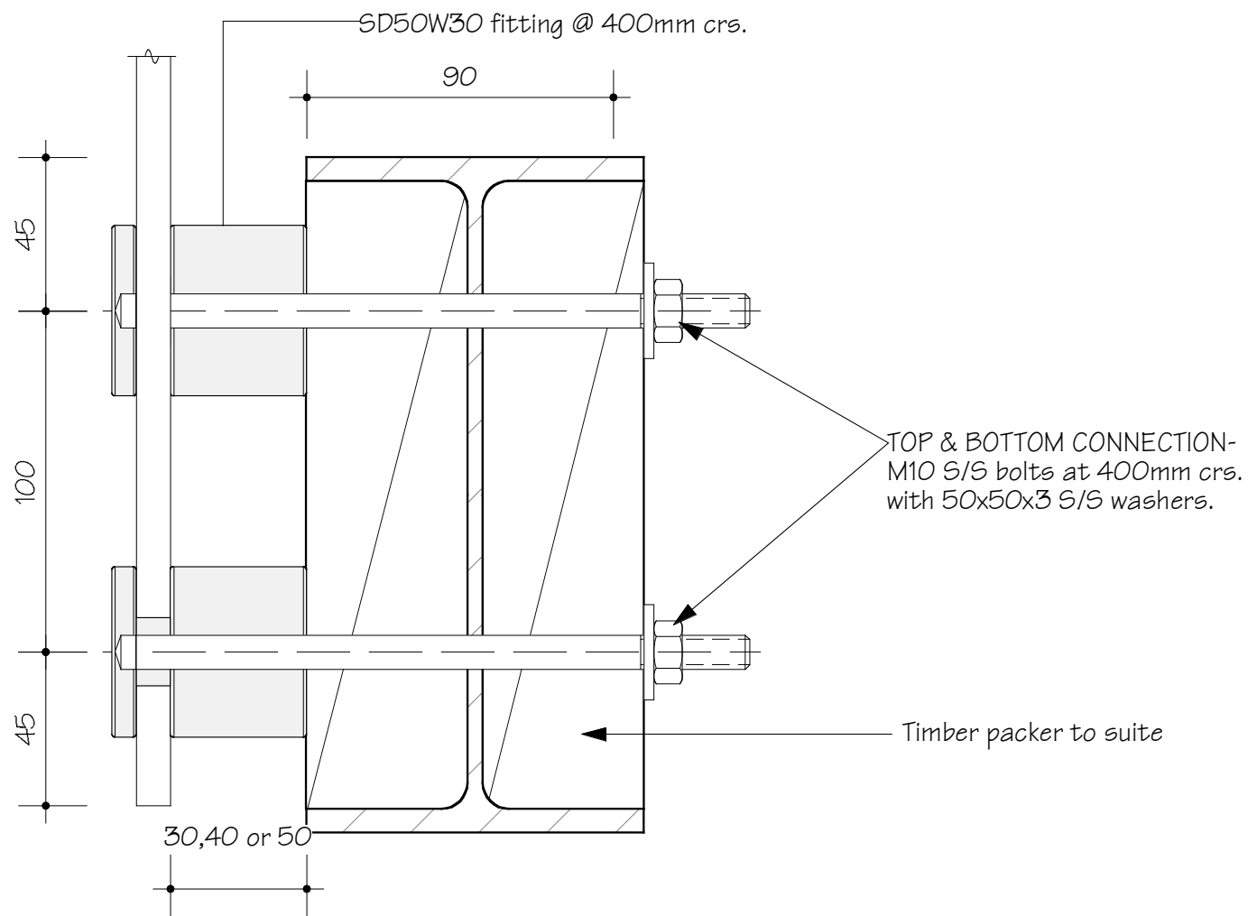
STEEL FIXING
