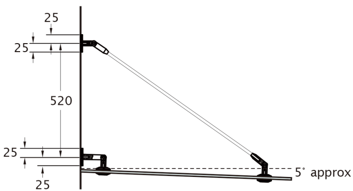
Glass Sloping Forward, Glass above wall bracket
