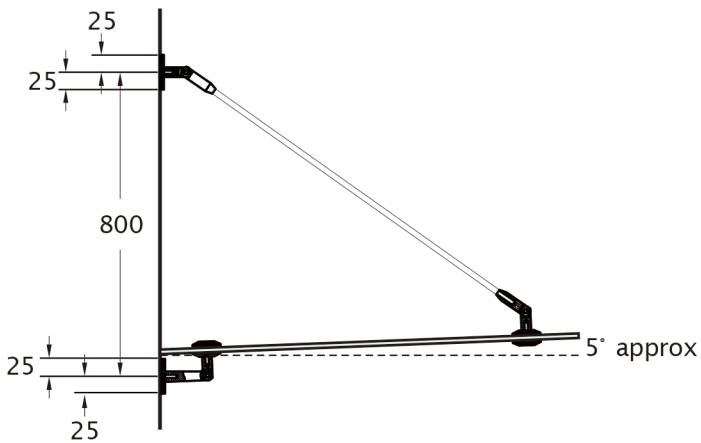
Glass Sloping Forward, Glass below wall bracket
