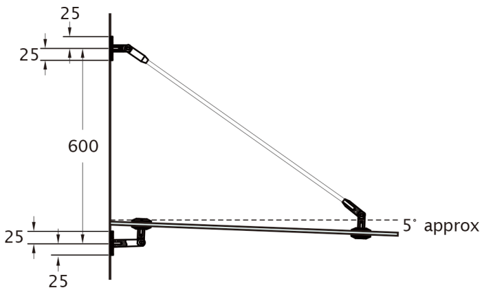
Glass Sloping Forward, Glass above wall bracket
